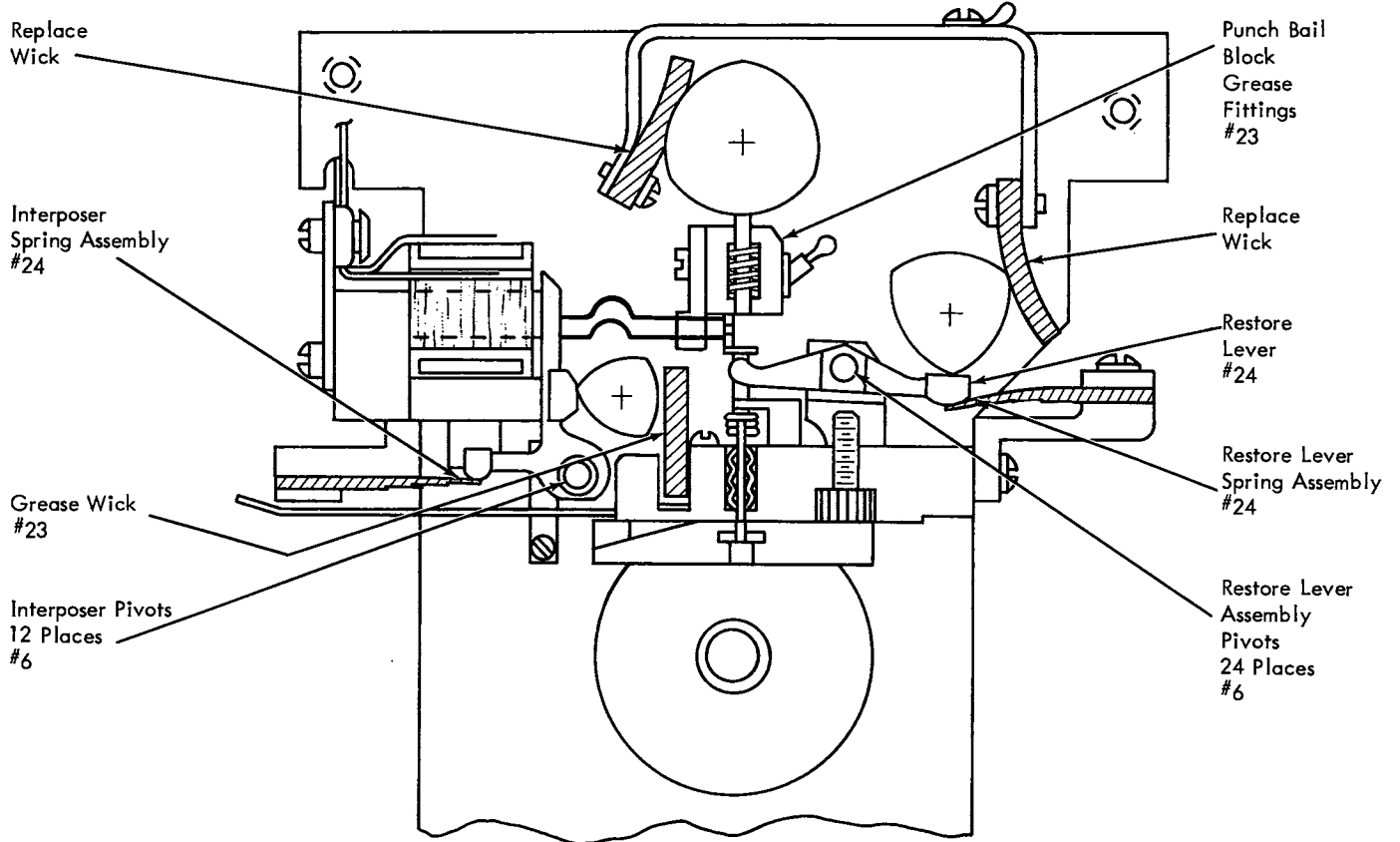
Figure 3-2. Punch Unit Lubrication
