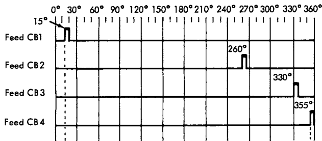
Figure 4-6. Feed CB Emitter Adjustment
