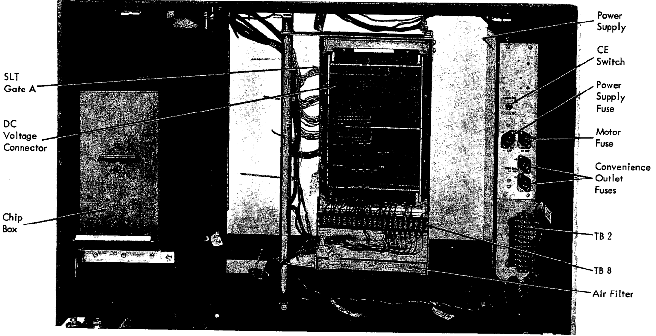
● Figure 6-3. IBM 1442 Models 5, 6, and 7 Locations (Below Base, Front View)
