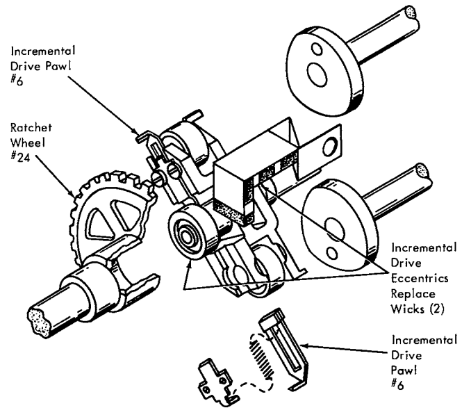
Figure 3-3. Incremental Drive Lubrication
