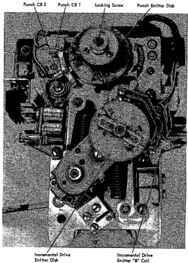
Figure 4-7. Punch and Incremental Drive Emitters
